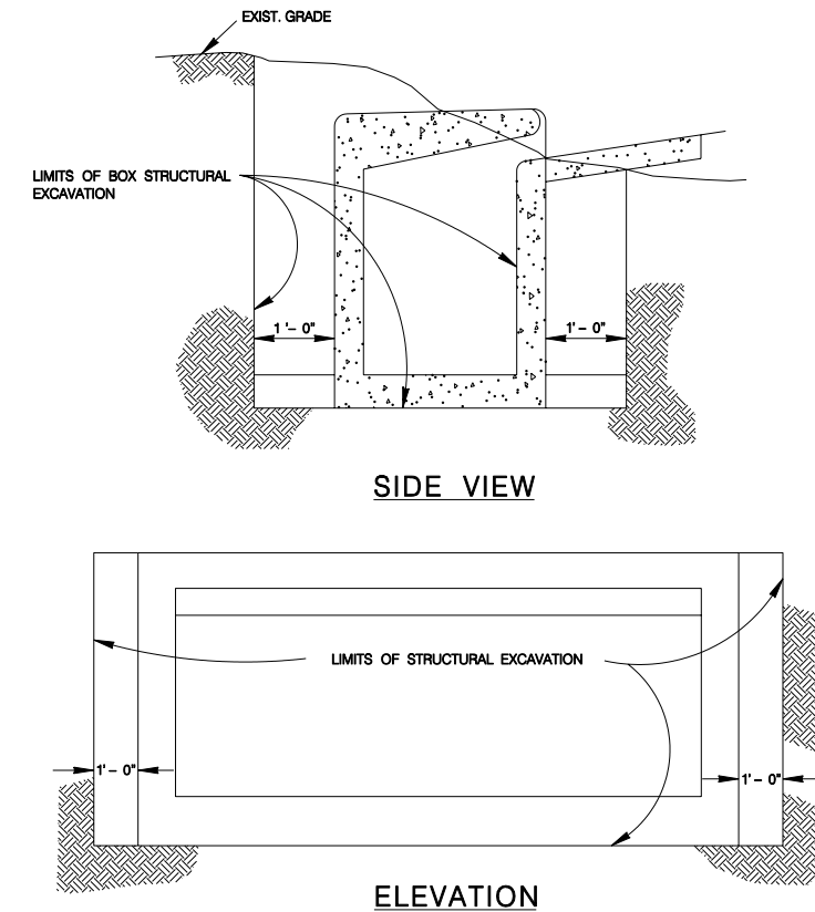
STRUCTURAL EXCAVATION AT JUNCTION BOXES NO SCALE
